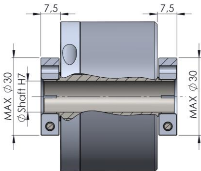
Shaft *M
